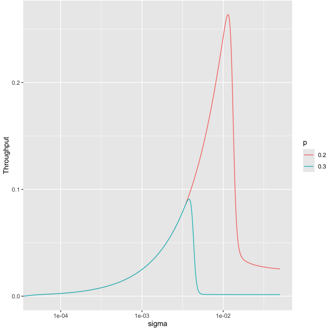
Figure 3: Theoretical slotted-ALOHA throughput for N = 25 and the two requested values of p .
