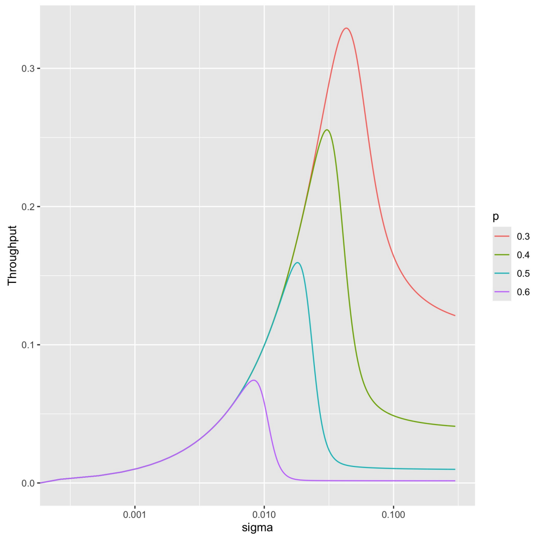
Figure 2: Theoretical slotted-ALOHA throughput for N = 10 and the four requested values of p .
